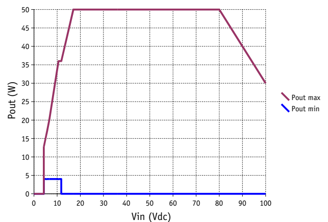
Figure 6 : PGDS-50-O-K Output Power versus Input Voltage
