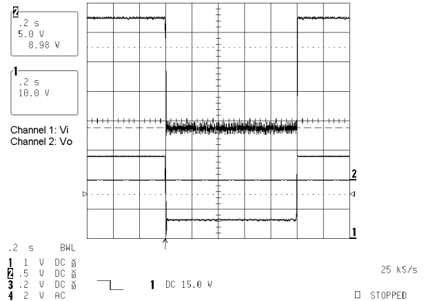
Figure 4 : PGDS-50-O-K Transient Response at 100Vdc
