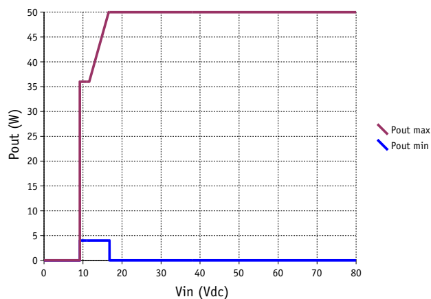
Figure 5 : PGDS-50-N-K Output Power versus Input Voltage
